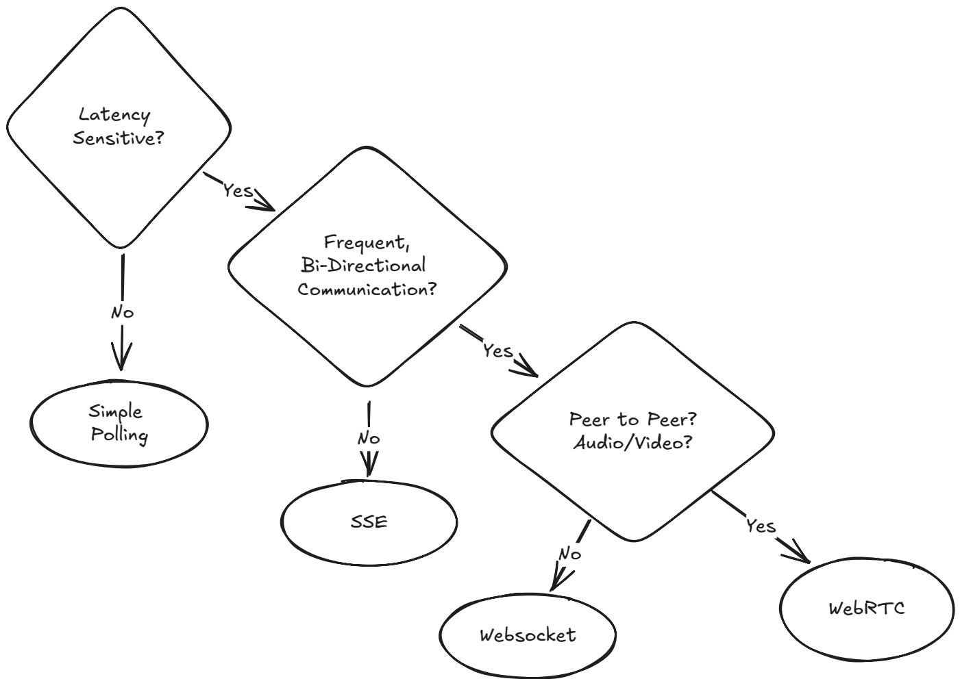
Client Updates Flowchart
