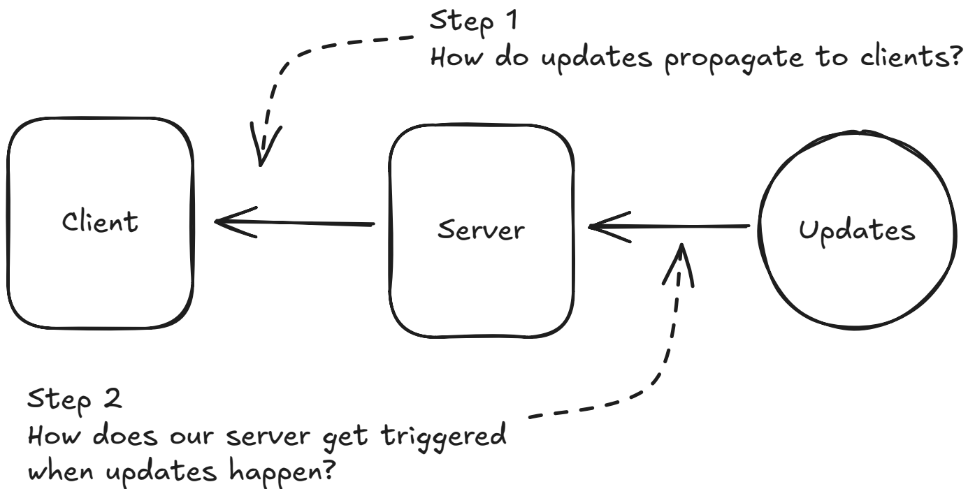
Two Hops for Real-time Updates
