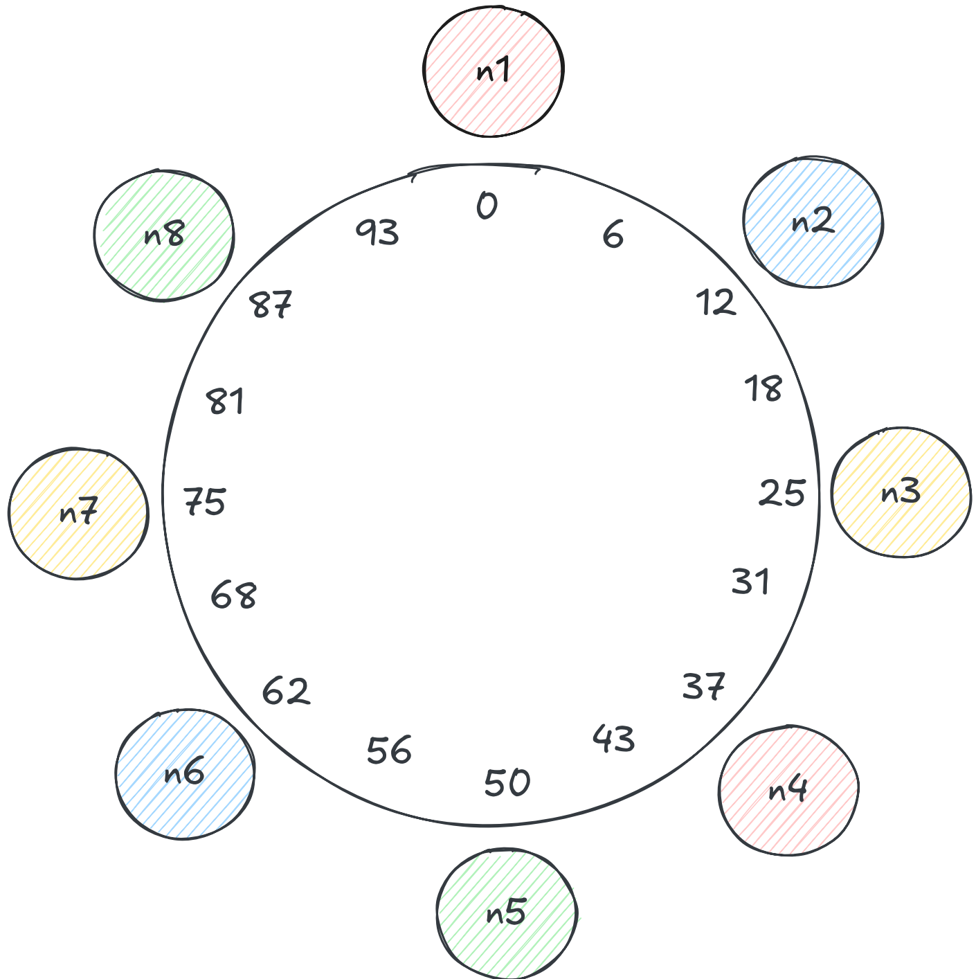
Consistent Hash Ring
