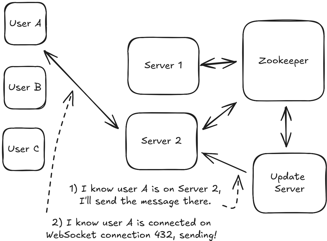
Sending Updates to the Right Server
