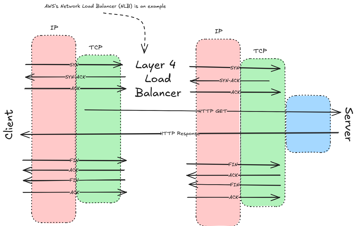
Simple HTTP Request with L4 Load Balancer
