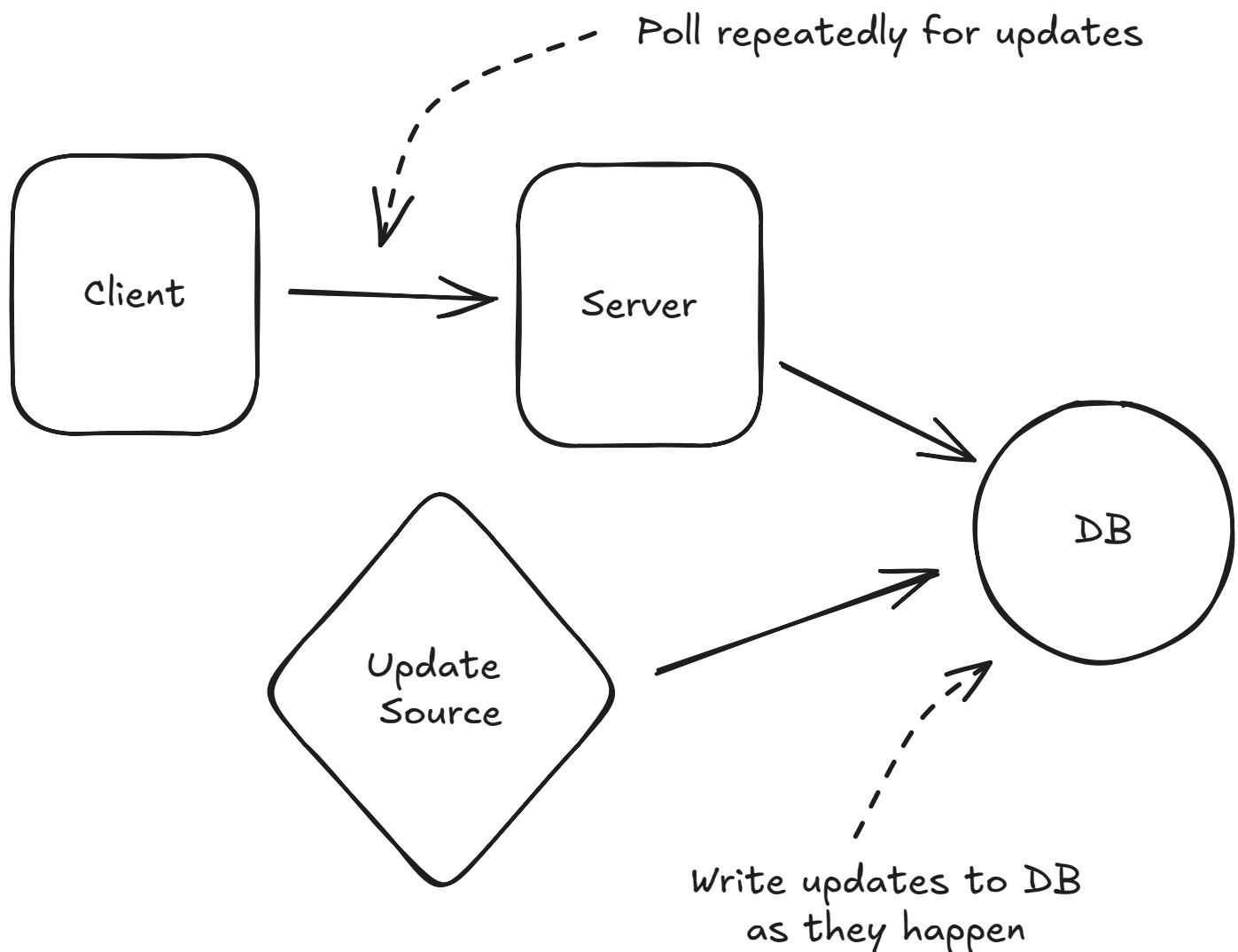
Pulling with Simple Polling
